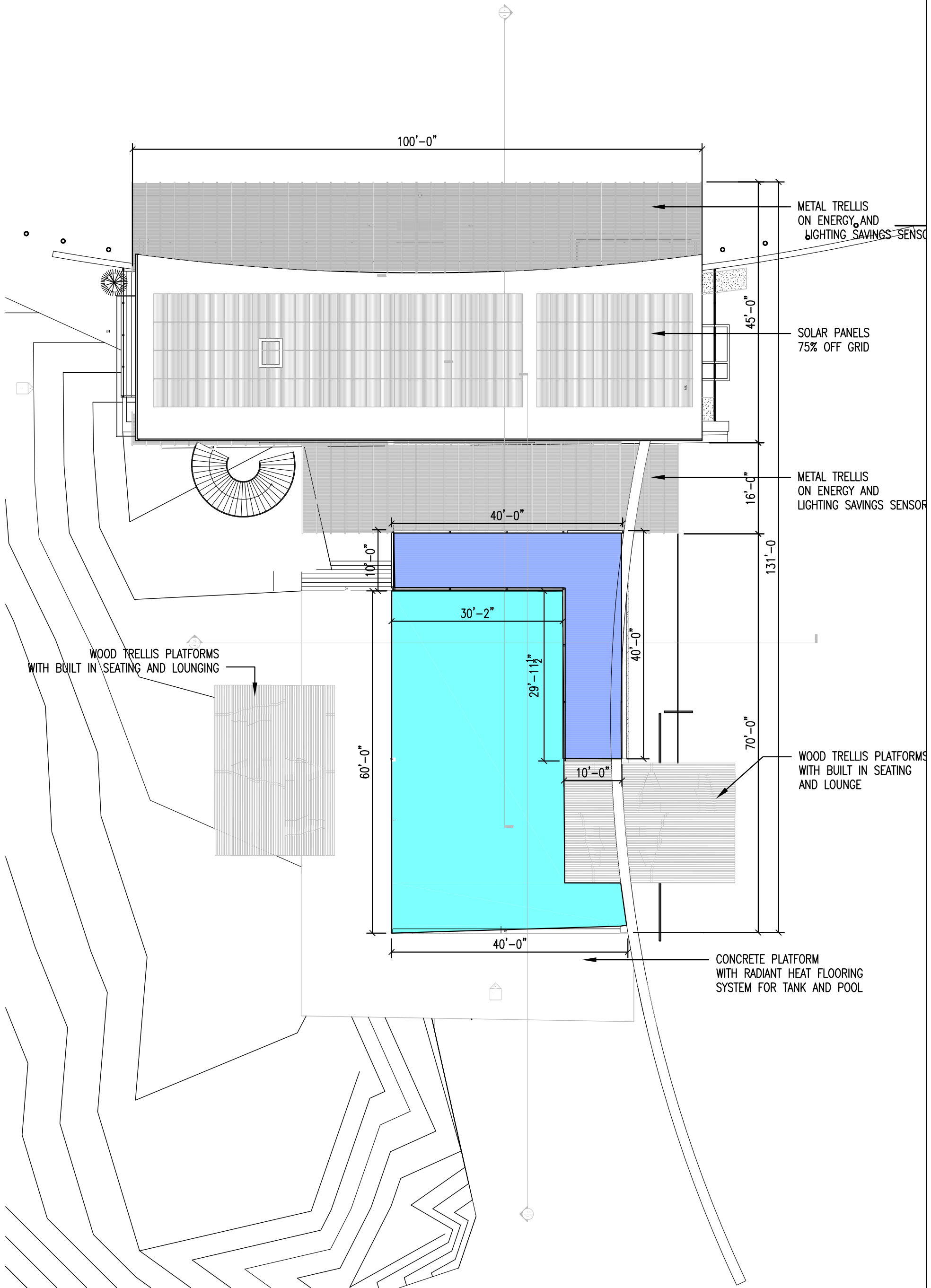
1 PLAN 1/16" = 1'-0"
